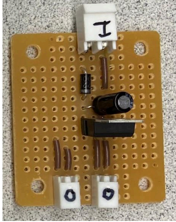
Image 18: 5V Voltage Regulator
