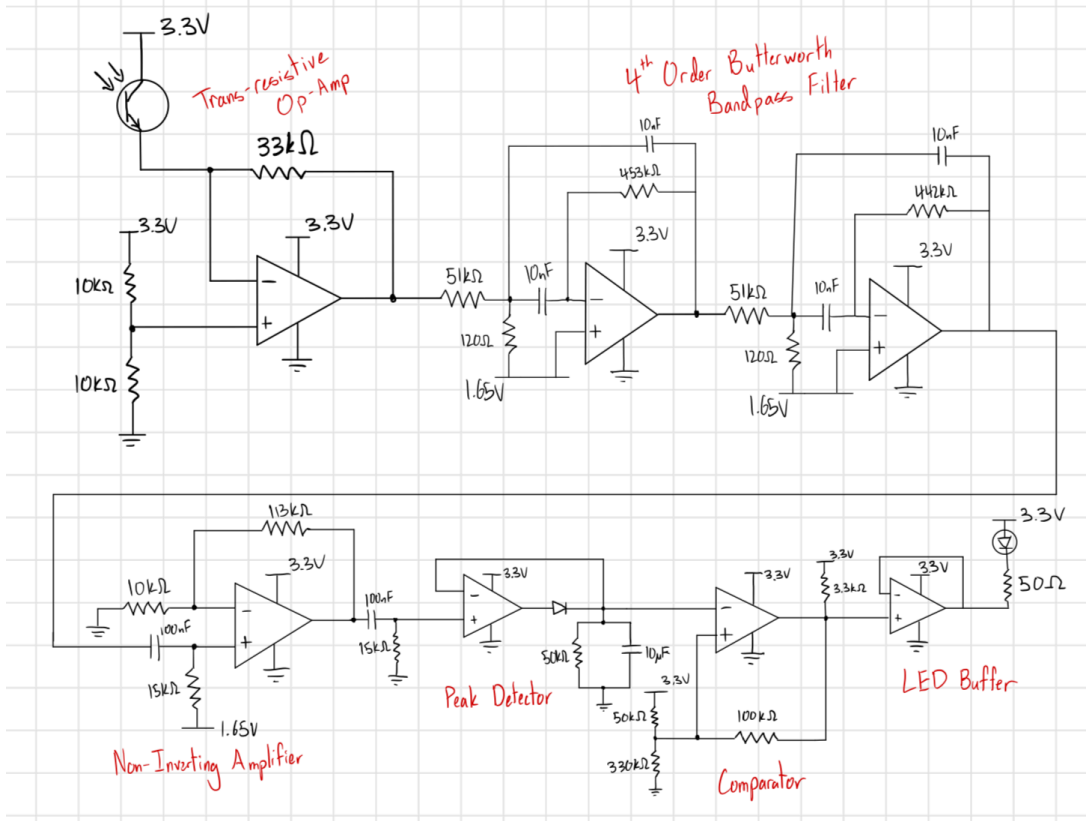
Image 19: Beacon Detector Schematic
