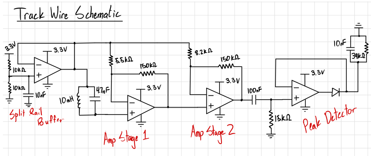
Image 14: Track Wire Schematic
