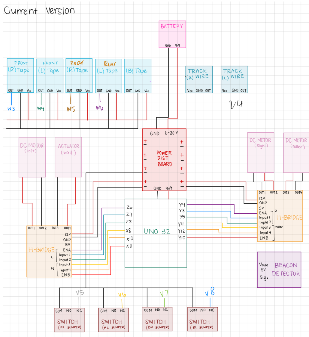
Image 17: Robot Component Pinout
