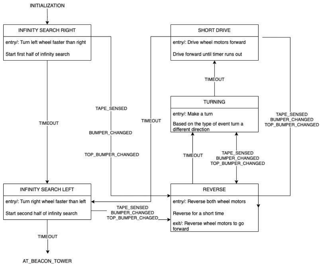
Image 22: Searching for Spheres Sub State Machine
