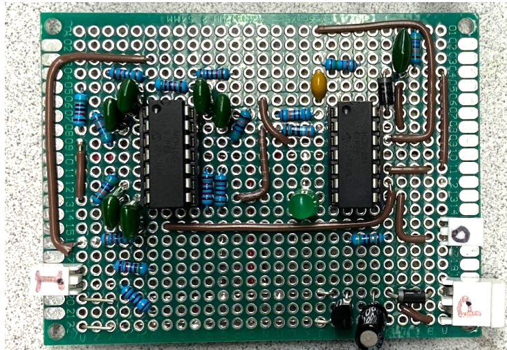
Image 20: Beacon Detector on Perfboard
