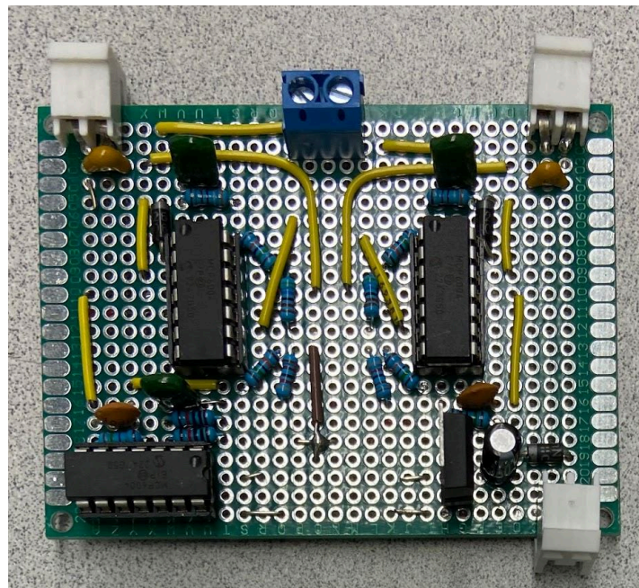
Image 15: Track Wire on Perfboard
