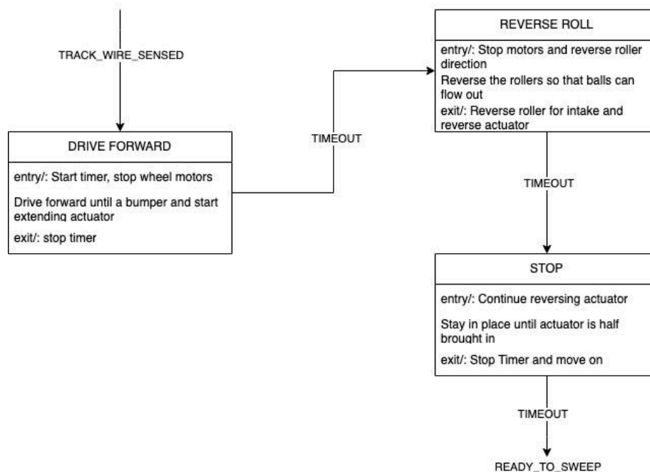
Image 24: Deposit Sub State Machine
