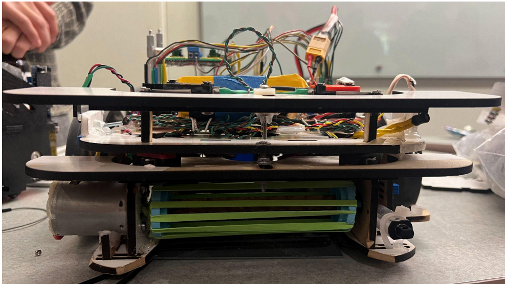
Image 10: Front View
