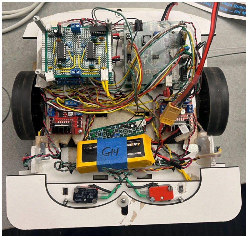
Image 12: Top View
