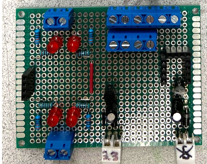
Image 16: Tape Sensor and Bump Switch Power Board
