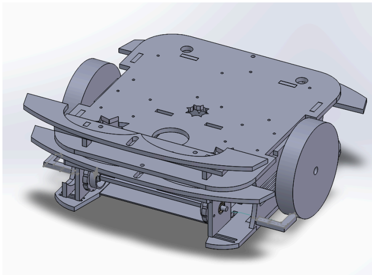
Image 3: Isometric Front View of the Autonomous Robot
