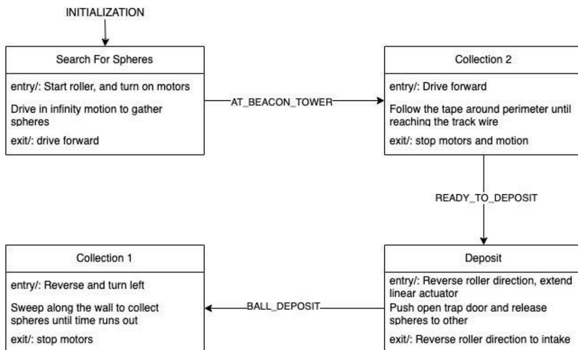
Image 21: Top Level Hierarchical State Machine
